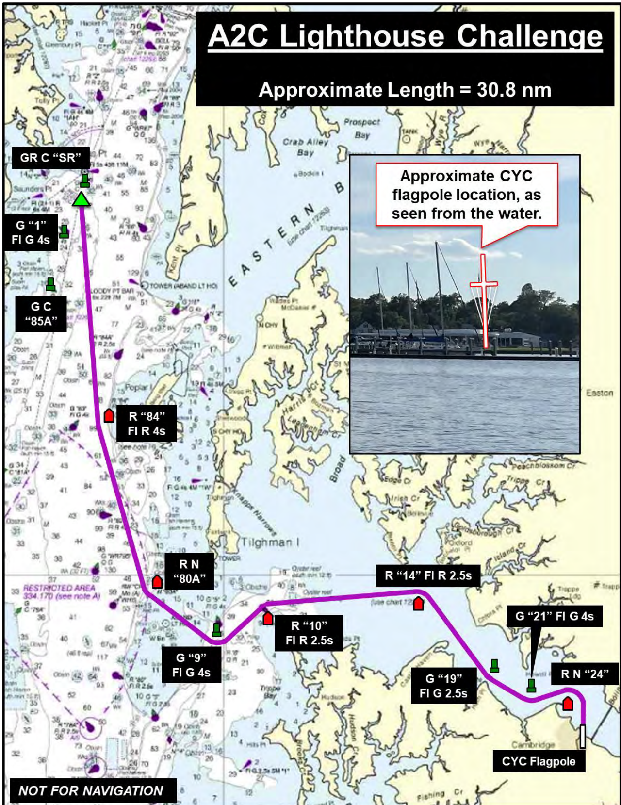
Figure 1. A2C Lighthouse Challenge Course Diagram
